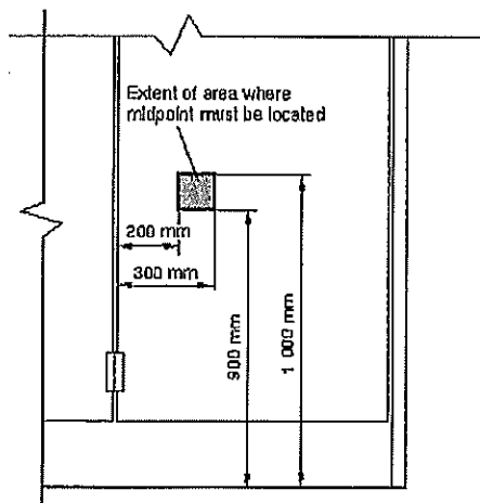
Figure A-3.8.3.8.(1)(b)(iv).A Door Pull Location
