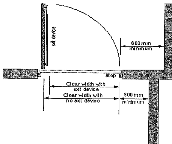
Figure A-3.8.3.3.(1) Clear Doorway Width
