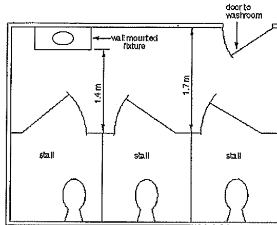
Figure A-3.8.3.8.(1) Water Closet Stalls
