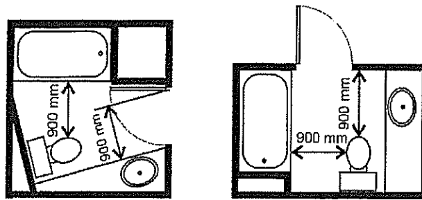
Figure A-3.8.3.3.(2) Residential Washrooms
