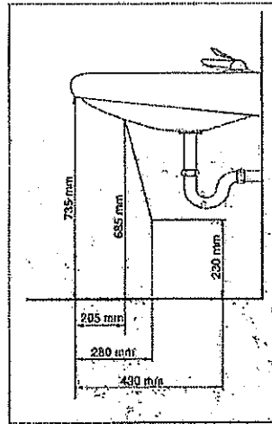
Figure A-3.8.3.11. Clearances Beneath a Lavatory
