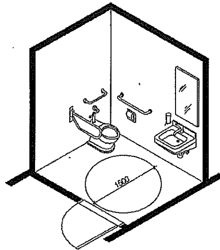
Figure A-3.8.3.12.B Universal Toilet Room with Outward Swinging Door
