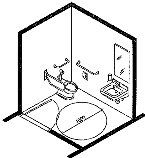
Figure A-3.8.3.12.A Universal Toilet Room with Inward Swinging Door
