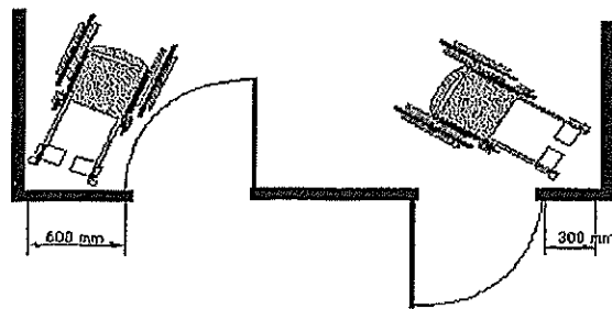
Figure A-3.8.3.3.(10) Doorway Clearance
