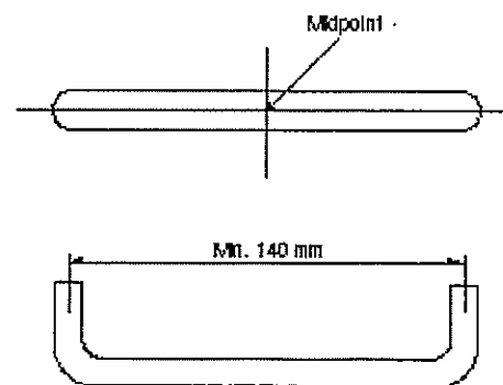
Figure A-3.8.3.8.(1)(b)(iv).B Door Pull Details
