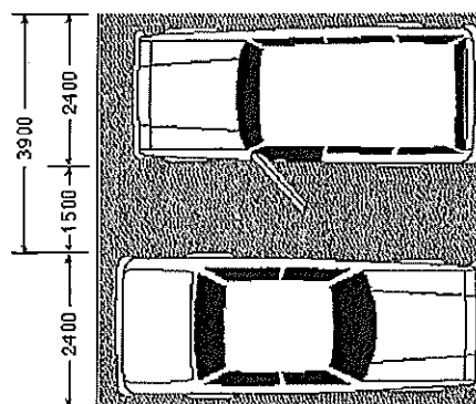
Figure A-3.8.2.2.B. Shared Access Aisle
