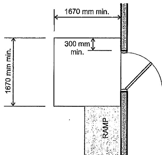
Figure A-3.8.3.4.(1)(c).B Landing Design at Doorway Leading to Ramps
