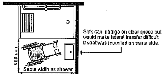
Figure A-3.8.3.13.(1)(b) Shower Design
