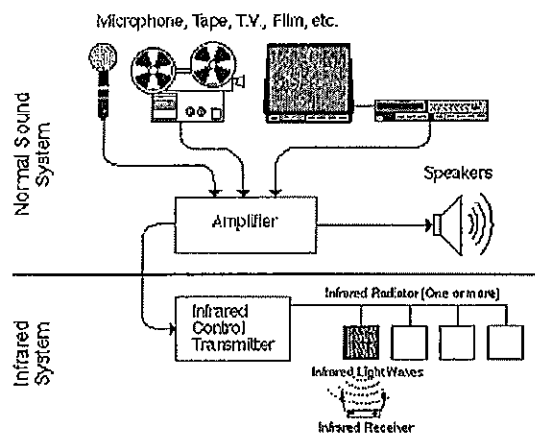
Figure A-3.8.3.7.B Infrared Sound Transmission System
