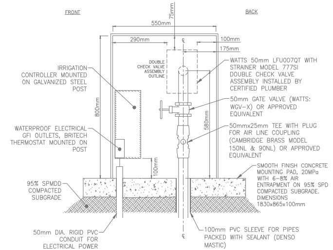
SECTION 'B - B' BACKFLOW PROTECTION ASSEMBLY
