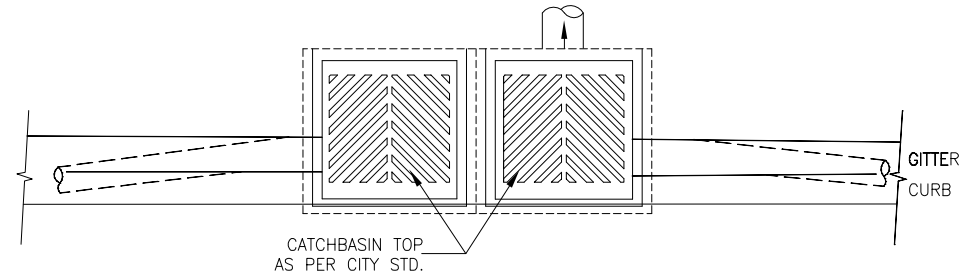
DOUBLE CATCHBASIN
