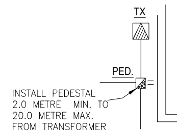
TYPICAL PLAN LAYOUT
