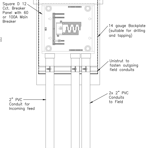
FRONT ELEVATION FRONT DOOR PANELS REMOVED
