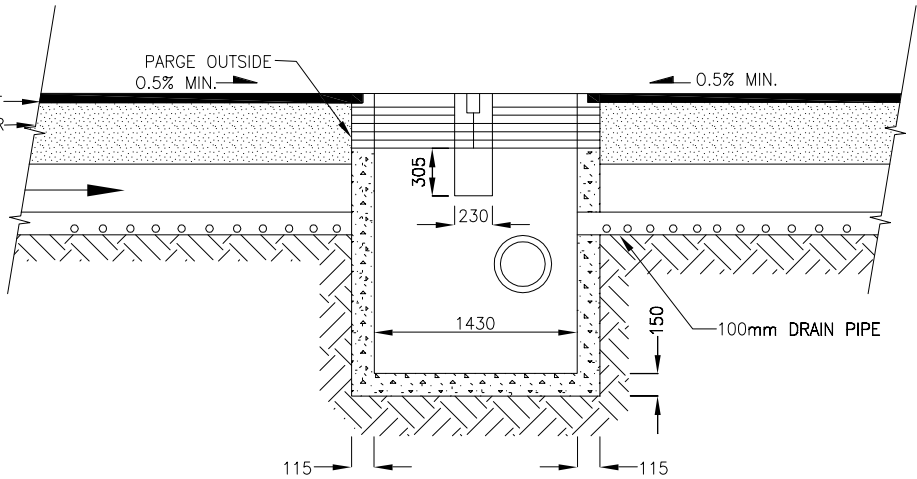
DOUBLE CATCHBASIN
