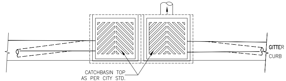
DOUBLE CATCHBASIN
