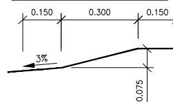
TRUCK APRON DETAIL
