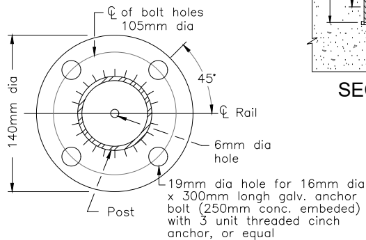
PLAN OF BASE PLATE
