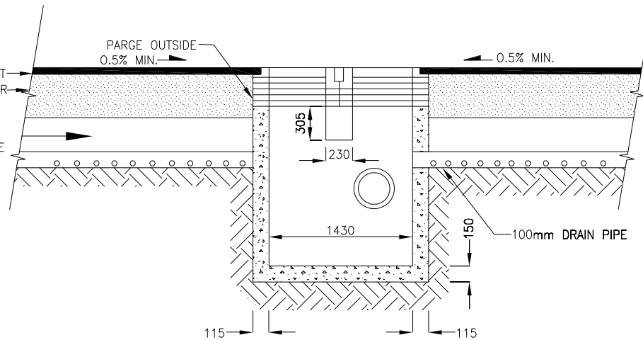
DOUBLE CATCHBASIN
