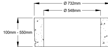
CONCRETE ADJUSTMENT UNIT
