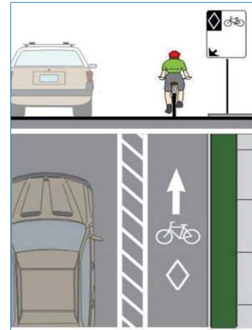
Buffered Bicycle Lane
