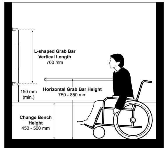
Figure 96b: Accessible Changing Stall - Elevation View
