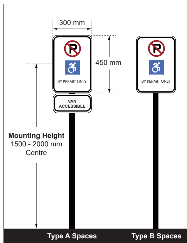
Figure 38: Accessible Parking Vertical Signage
