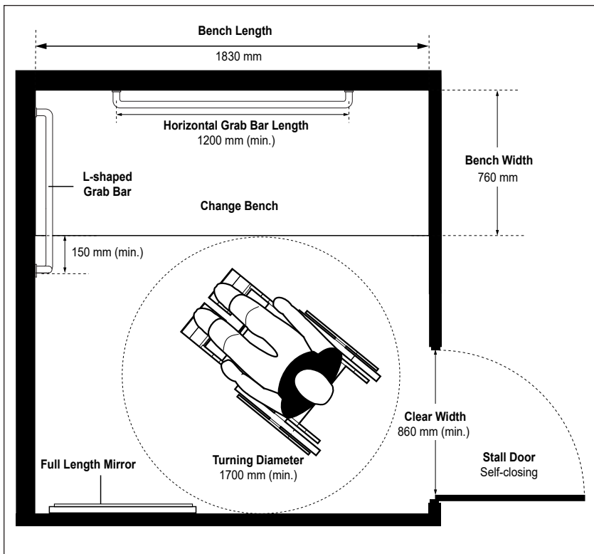
Figure 96a: Accessible Changing Stall - Plan View
