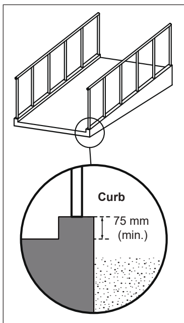
Figure 16a: Curb Protection
