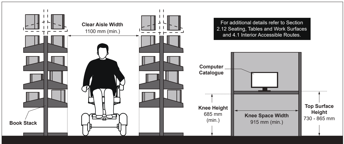
Figure 92: Book Stacks and Accessible Workstation - Elevation View
