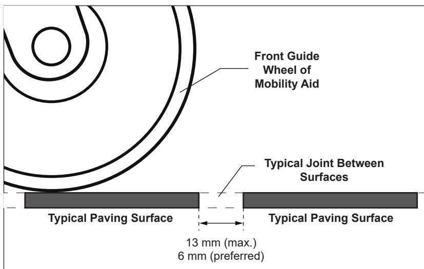
Figure 13: Joints Between Surfaces - Section View
