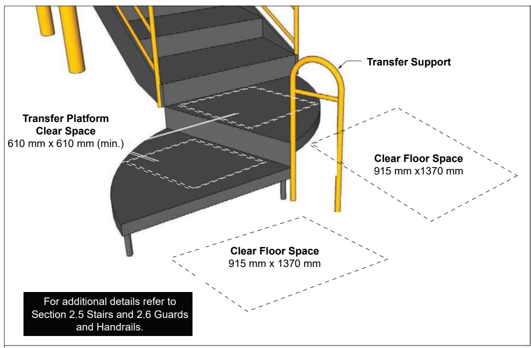
Figure 106: Transfer Systems
