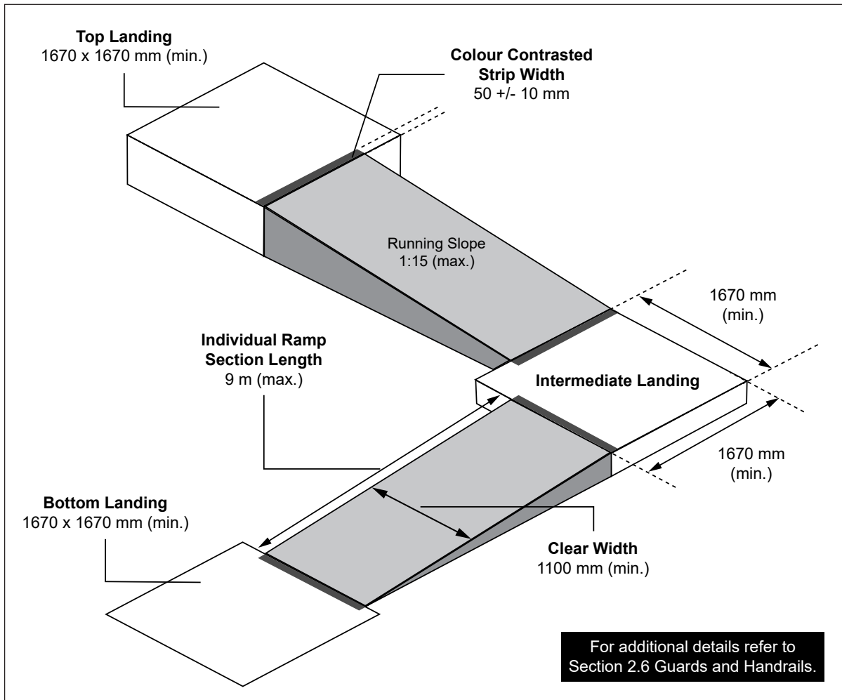
Figure 15: Ramp Design Features
