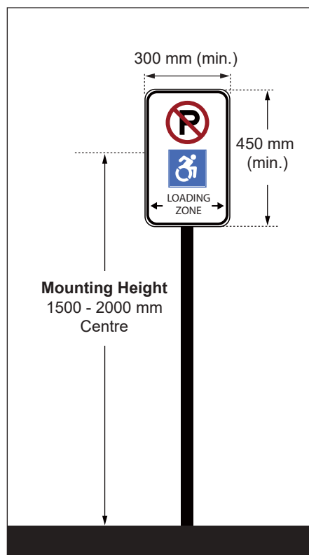
Figure 41: Passenger Loading Zone Vertical Signage
