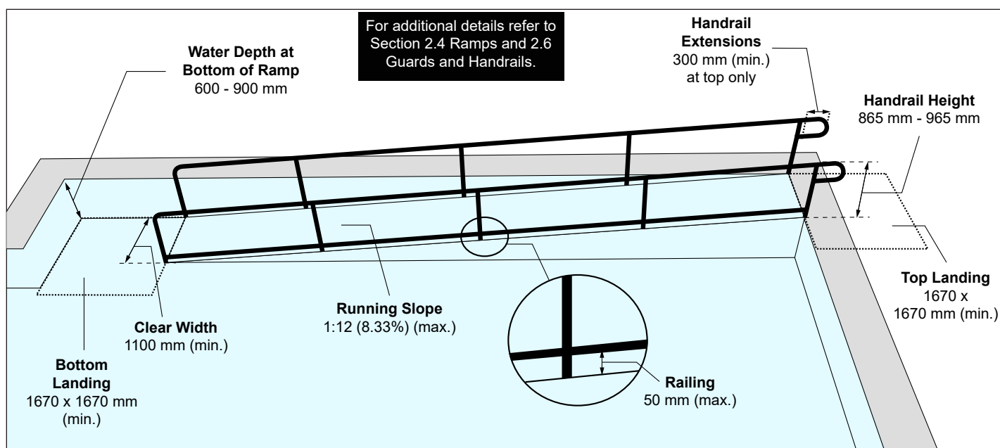
Figure 94: Sloped Entry or Ramp to Swimming Pool
