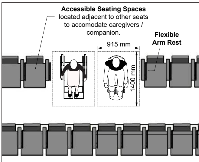
Figure 80: Accessible Seating Space Dimensions
