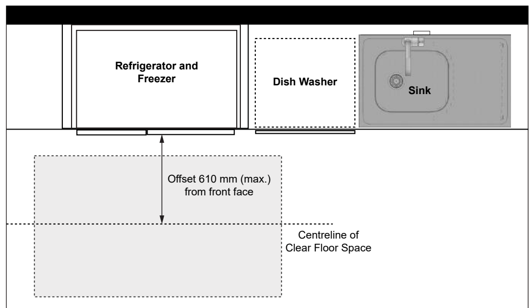
Figure 89: Clear Floor Space at Refrigerators and Freezers
