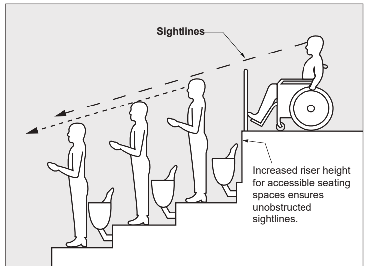
Figure 81: Lines of Sight
