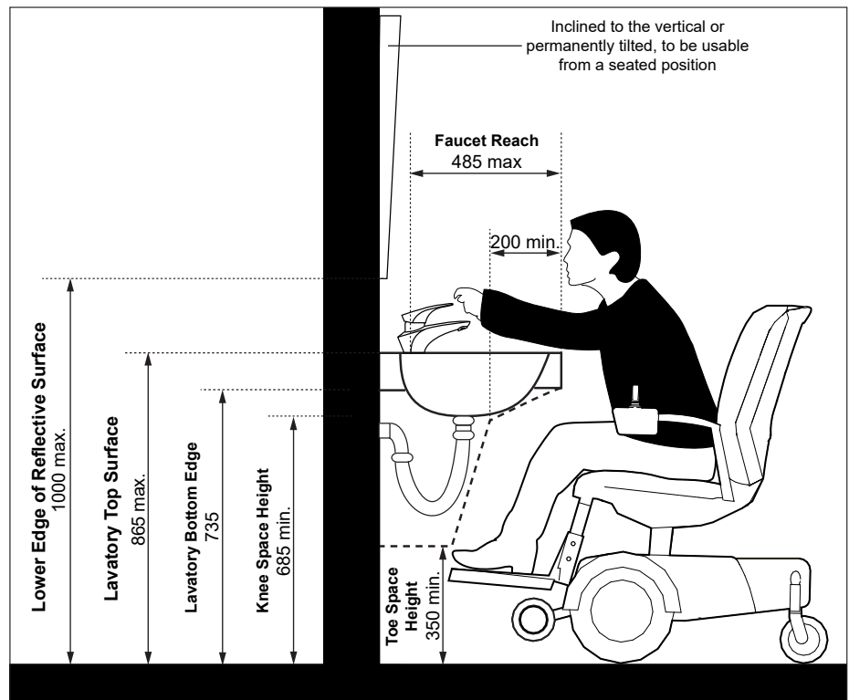
Figure 59a: Lavatories - Section View
