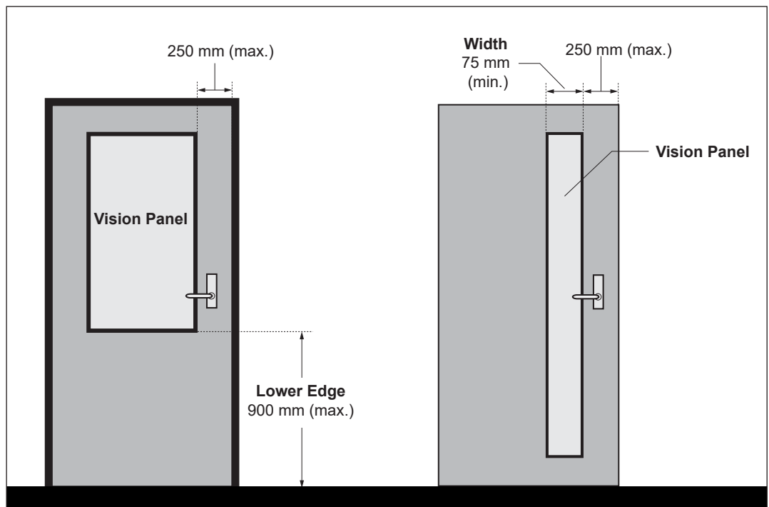
Figure 12: Vision Panels - Elevation View
