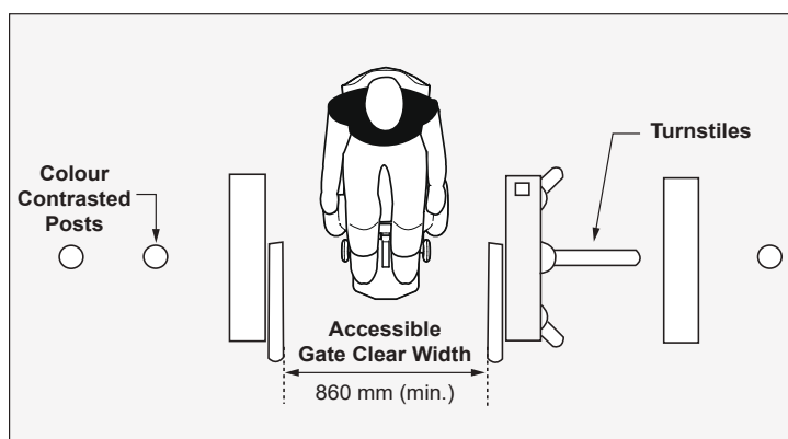
Figure 3: Accessible Controlled Gate
