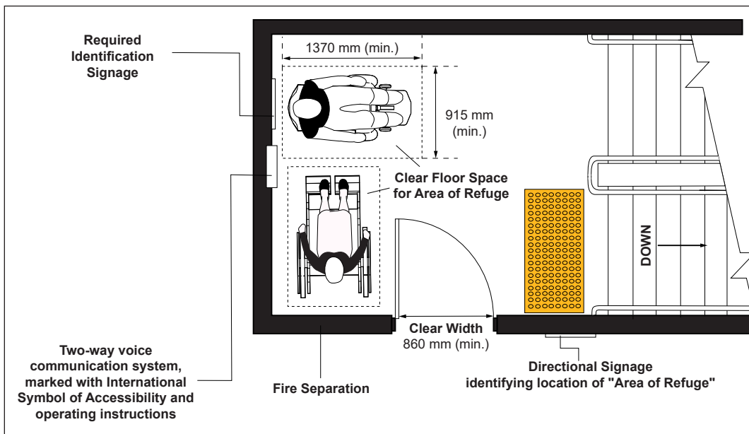
Figure 70: Example of Area of Refuge at Exit Stair
