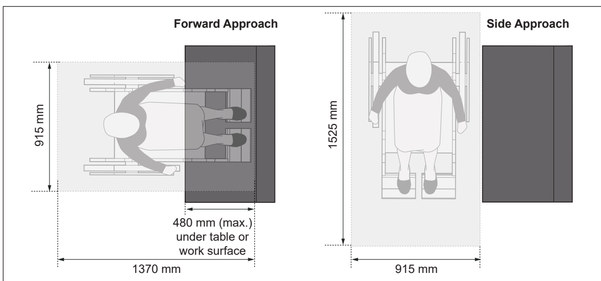
Figure 36b: Clear Floor Space Requirements and Approach at Tables and Work Surfaces - Plan View
