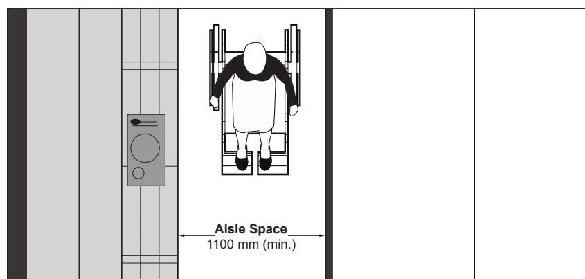
Figure 84b: Aisle Width - Plan View
