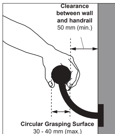
Figure 25a: Handrails on Wall
