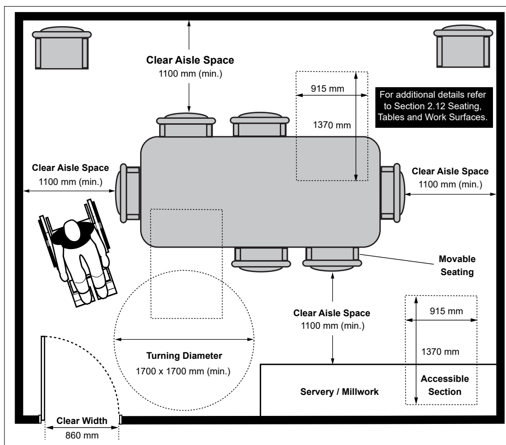
Figure 83: Typical High-Use Meeting Room Design and Layout
