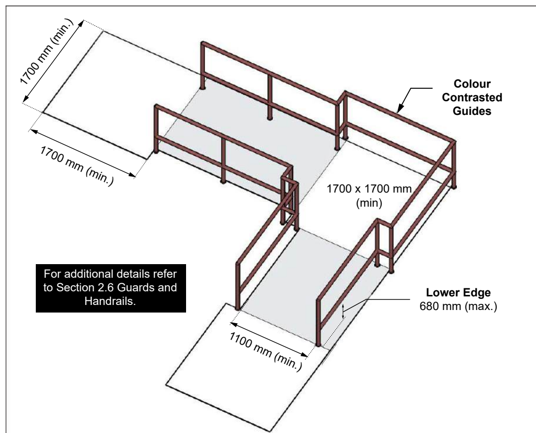
Figure 100: Fixed Queuing Guides
