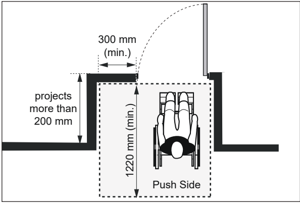
Figure 8b: Push Side Approach at Recessed Side-Hinged Door - Plan View
