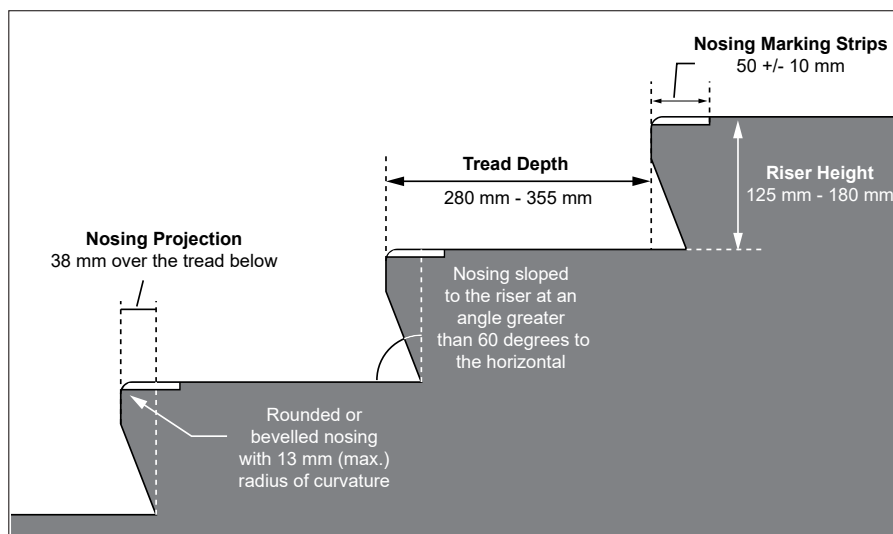
Figure 22: Stair Design Features - Section View
