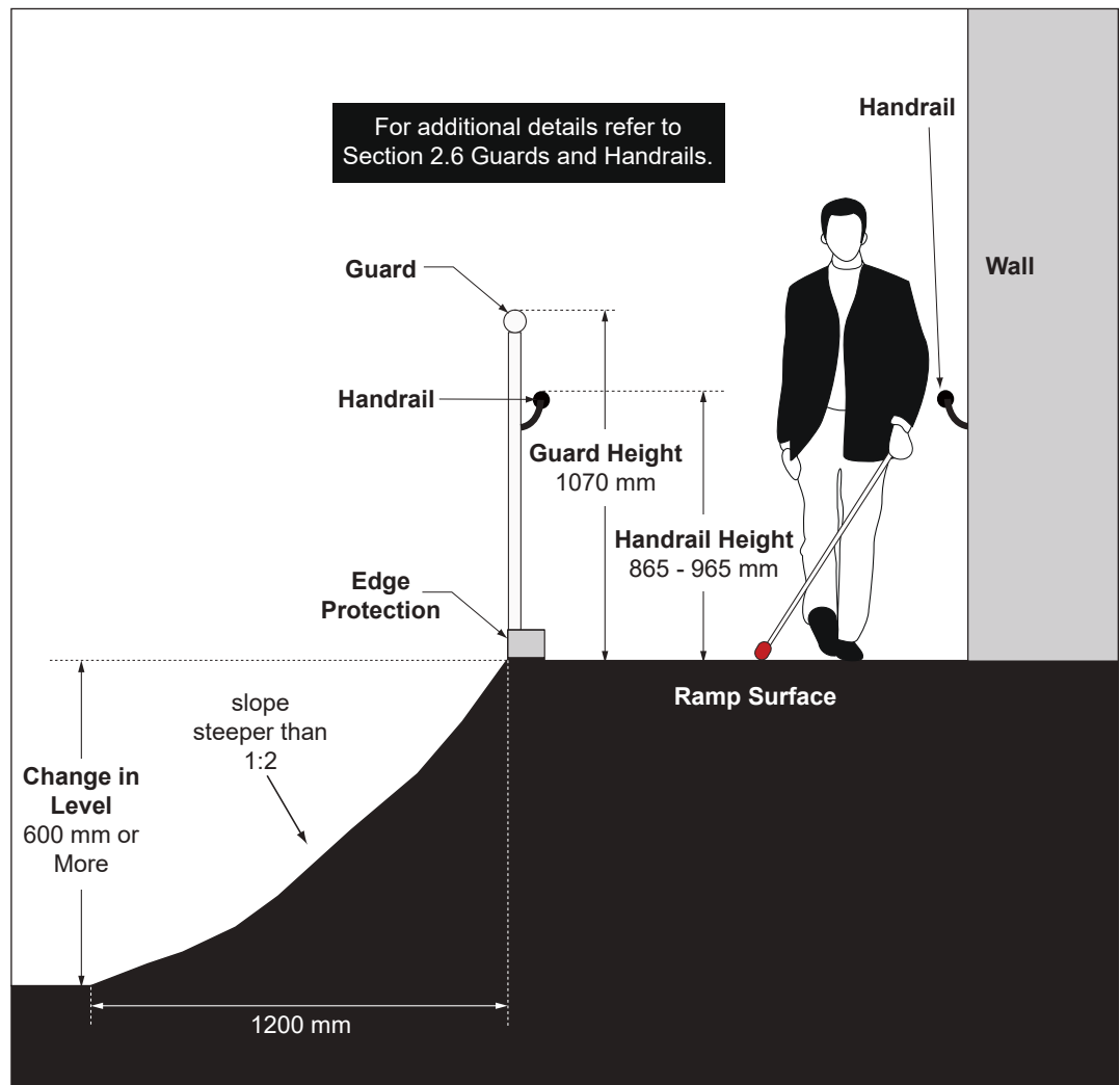
Figure 21: Guard Provision at Ramp - Section View
