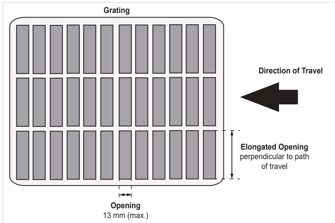
Figure 14a: Grating Opening - Plan View
