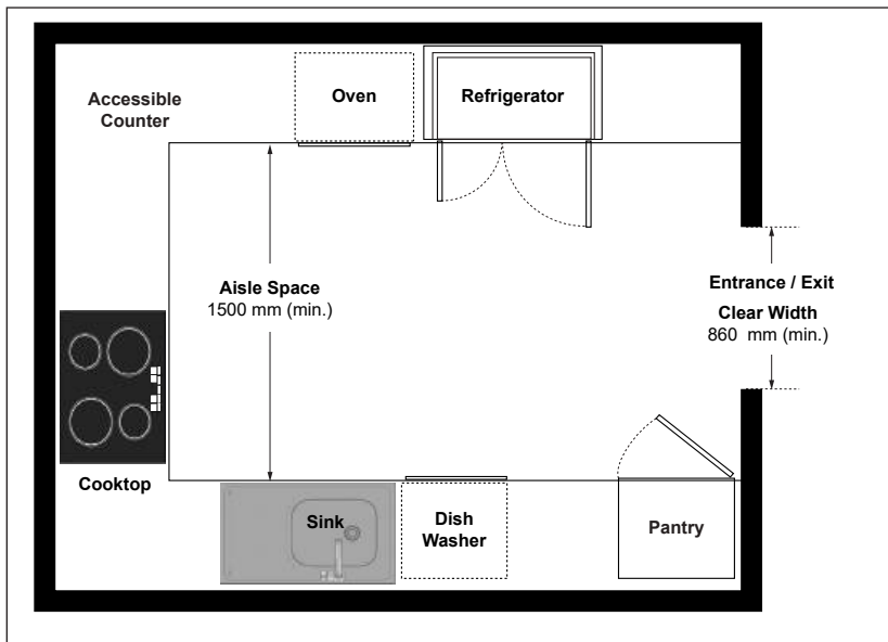
Figure 86: U-Shaped Kitchen - Plan View
