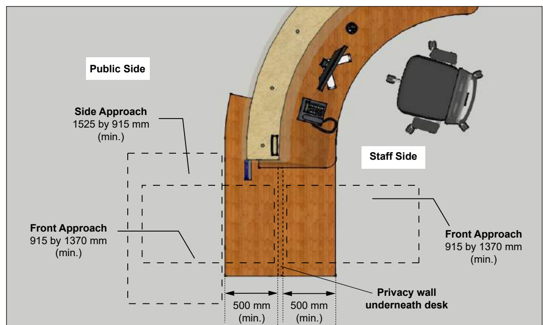
Figure 98a: Clear Floor Space Requirement at Accessible Service Counter - Plan View
