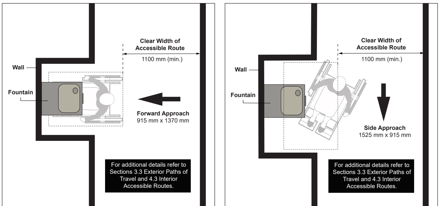
Figure 31: Clear Floor Space Requirements and Approach at Recessed Drinking Fountain - Plan View
