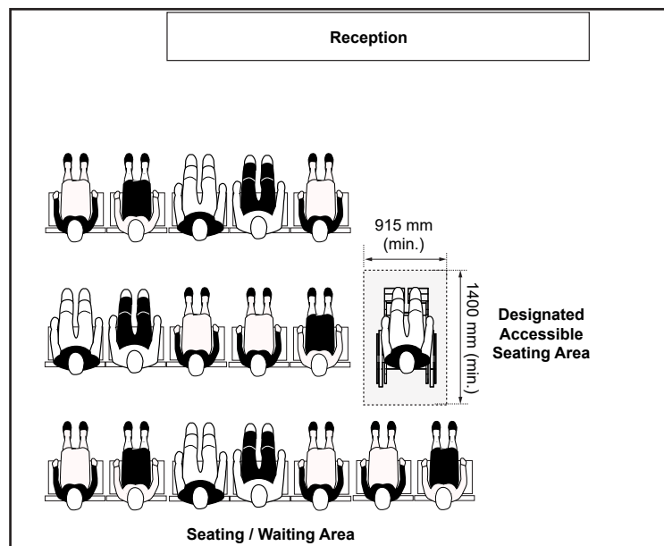
Figure 99: Waiting Area - Plan View
