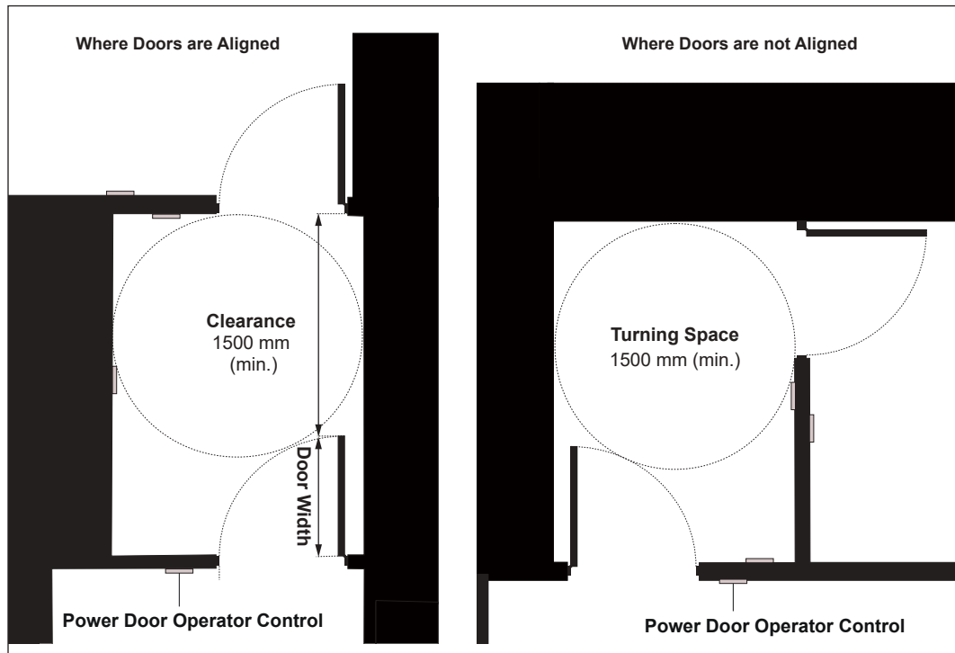
Figure 10: Doors in Series - Plan View
