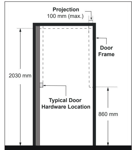
Figure 2b: Clear Width of Door - Section View
