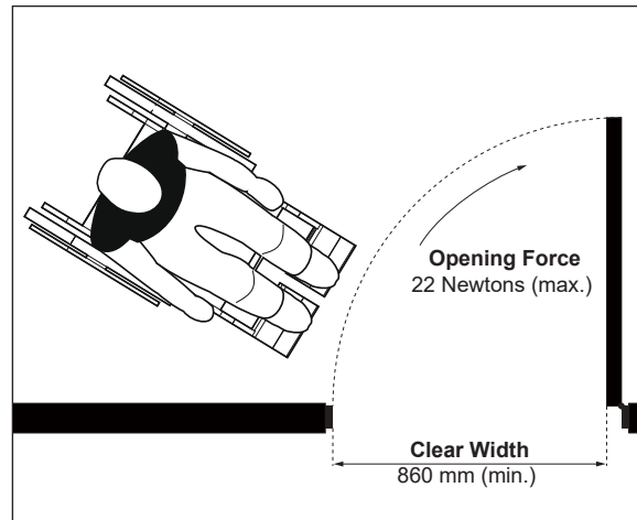
Figure 2a: Clear Width of Door - Plan View
