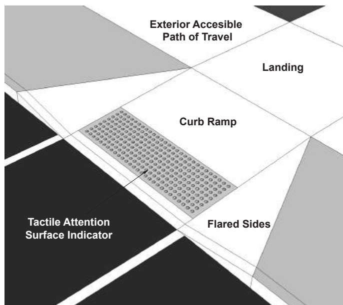
Figure 44a: Curb Ramp with Flared Sides
