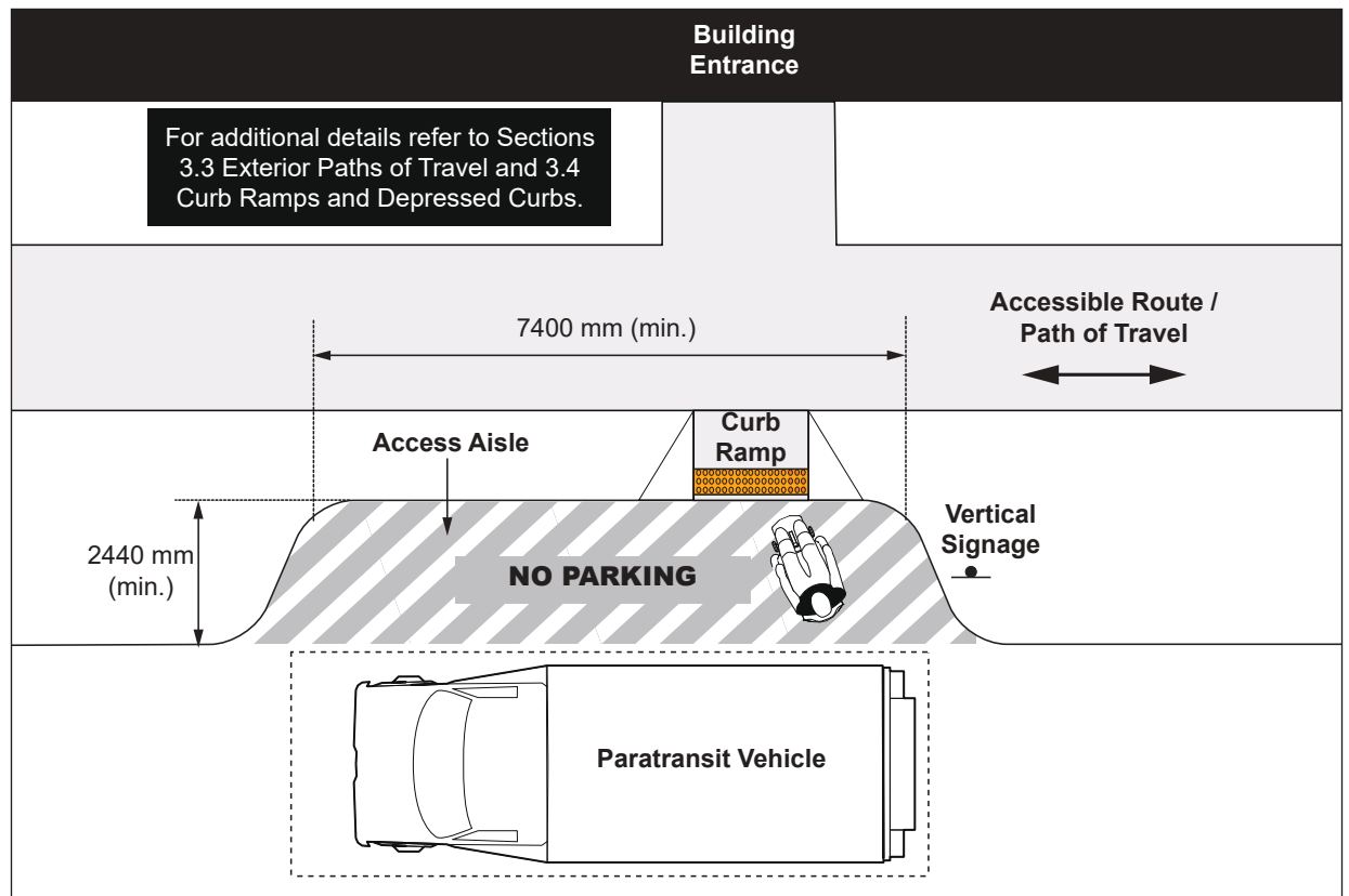
Figure 40: Passenger Loading Zone - Plan View
