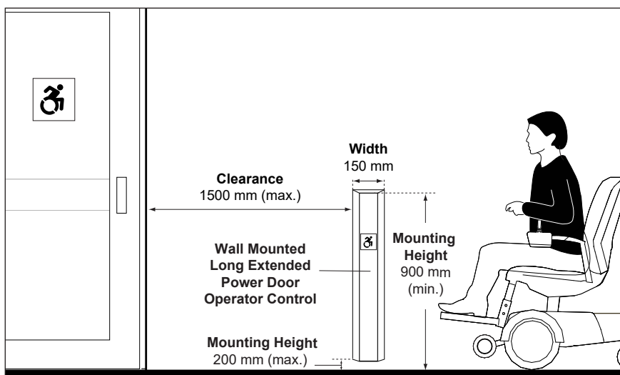
Figure 5b: Long Extended Power Door Operator - Elevation View
