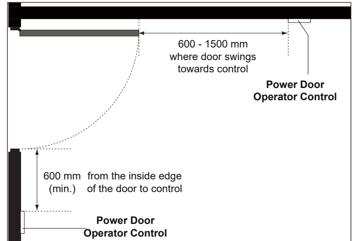
Figure 6: Power Door Operator Control Mounting Location - Plan View
