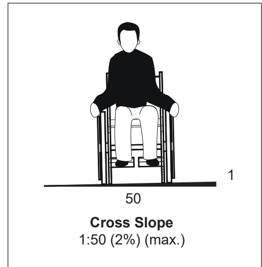
Figure 51: Cross Slope
