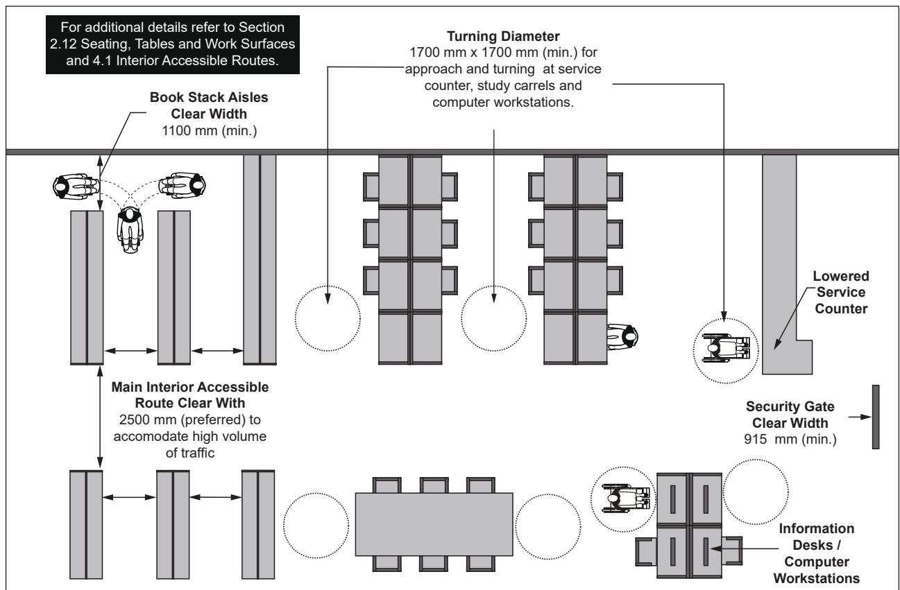
Figure 90: Library Design and Layout - Plan View
