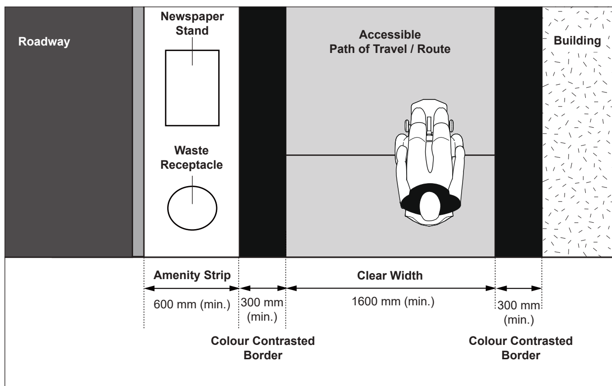
Figure 47: Typical Amenity Strip for Street Furniture Placement
