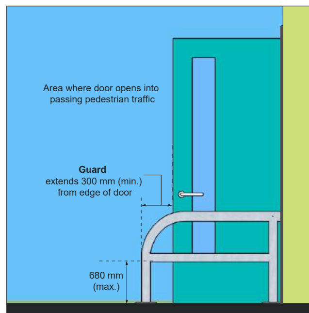
Figure 7b: Guard at Door - Elevation View
