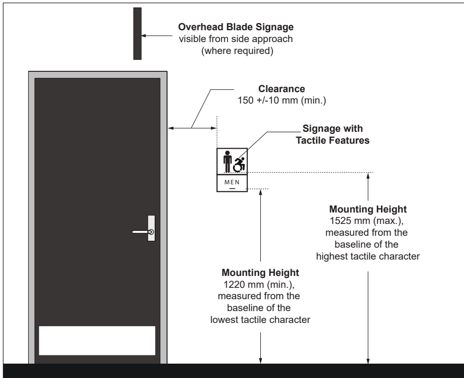
Figure 75: Mounting Location of Signage with Tactile Features - Elevation View
