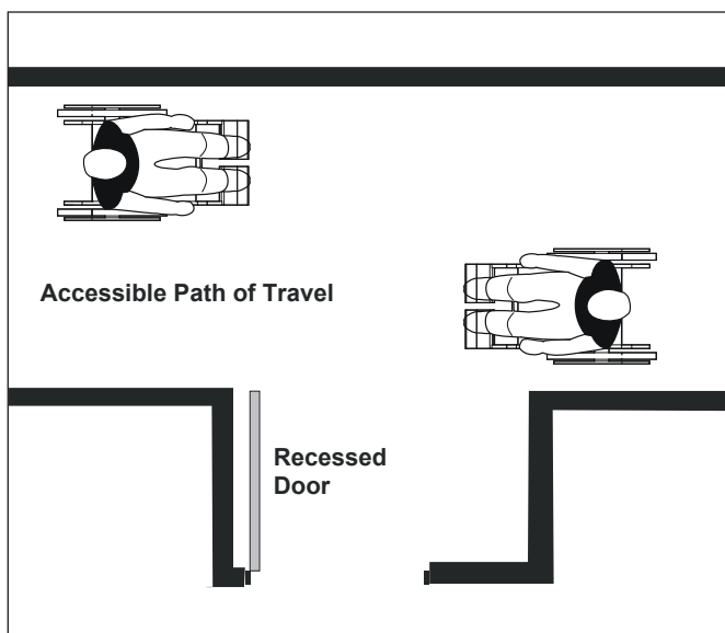
Figure 7a: Recessed Door - Plan View
