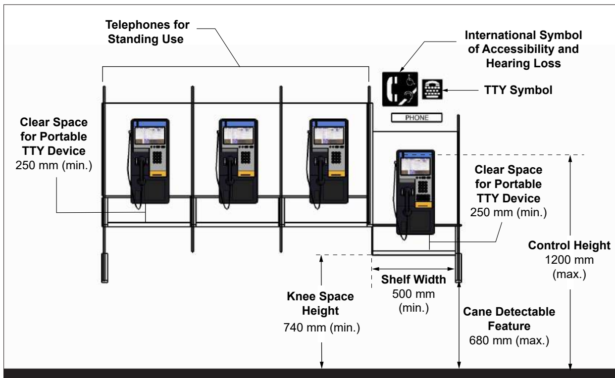
Figure 34: Public Telecom Amenity Provision and Layout
