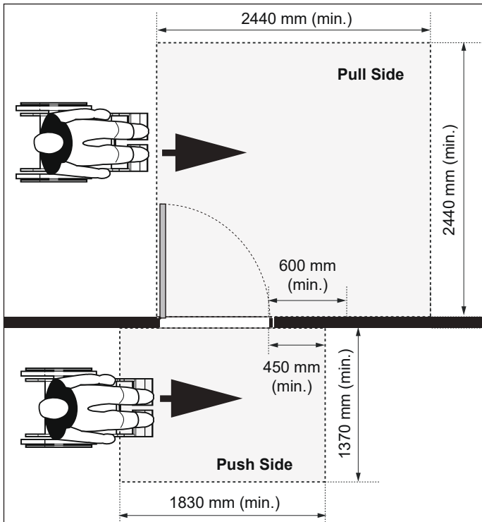
Figure 9c: Hinge Side Approach at Side-Hinged Door - Plan View
