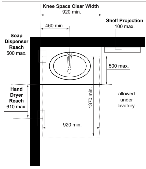
Figure 59b: Lavatories - Plan View
