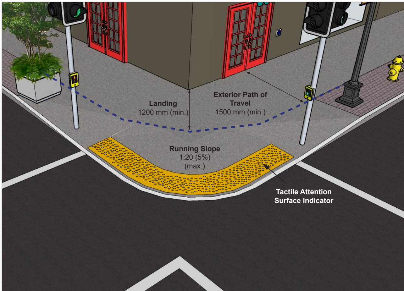
Figure 46: Typical Depressed Curb
