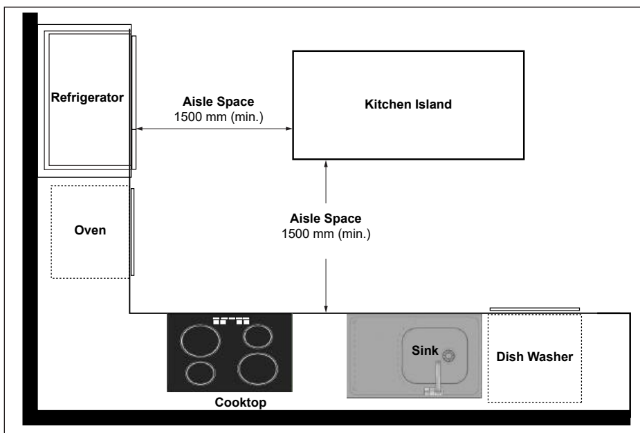
Figure 87: L-Shaped Kitchen - Plan View
