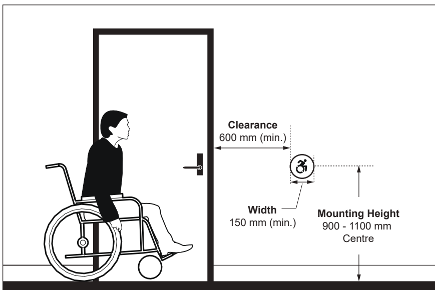
Figure 5a: Circular Push Button - Elevation View
