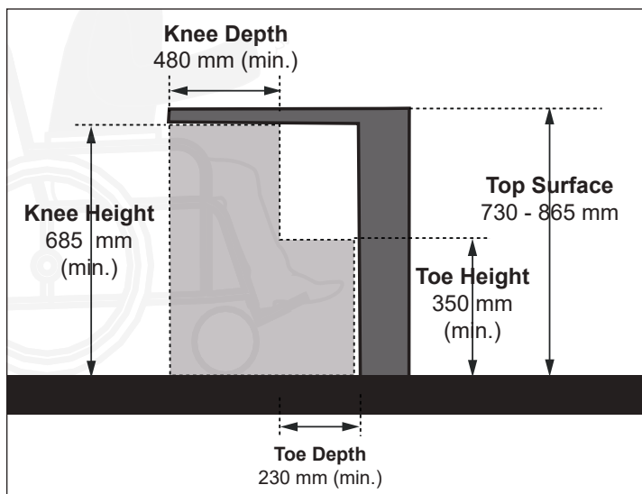
Figure 36a: Knee and Toe Clearances at Tables or Work Surfaces- Elevation View
