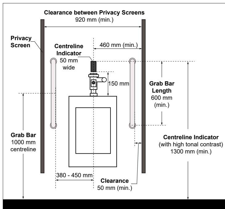
Figure 62b: Urinal - Front Elevation View
