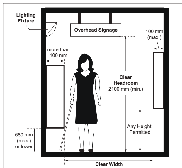
Figure 27: Protruding Objects
