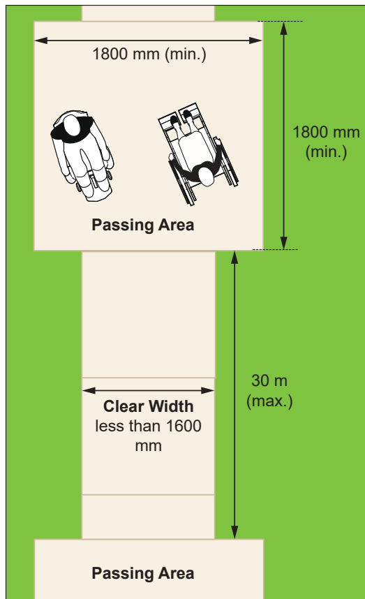
Figure 40b: Reduced Clear Width and Required Passing Area
