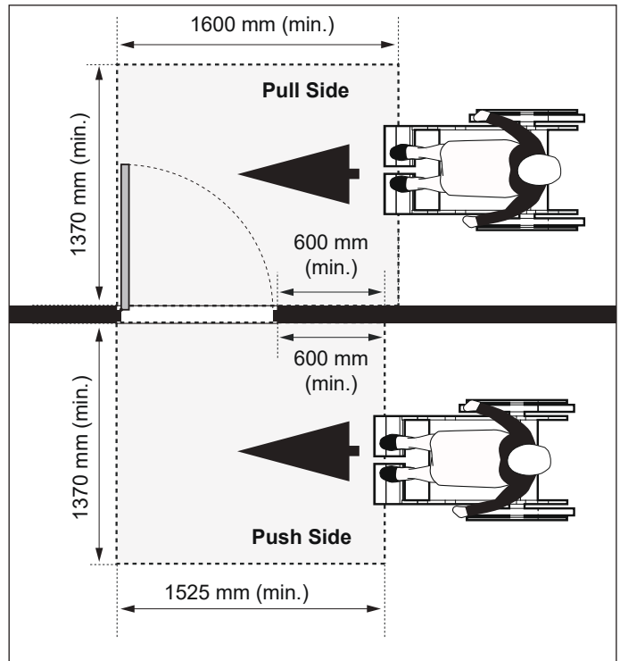
Figure 9d: Latch Side Approach at Side-Hinged Door - Plan View
