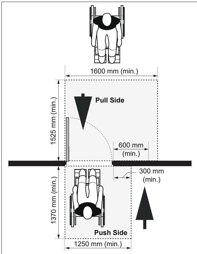
Figure 9a: Front Approach at Side-Hinged Door - Plan View
