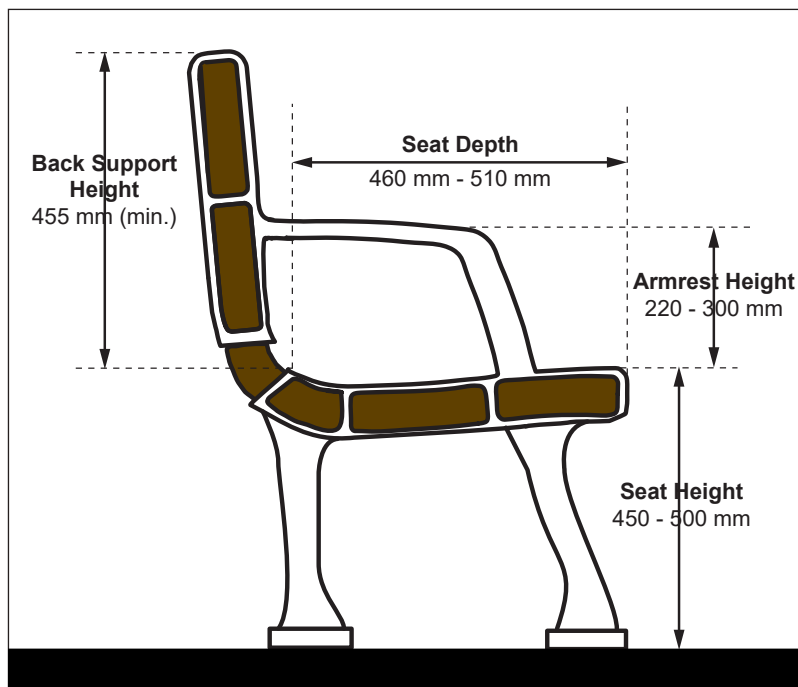
Figure 35: Typical Accessible Bench Dimensions - Section View
