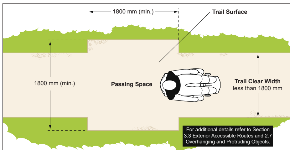
Figure 104: Trail Clear Width
