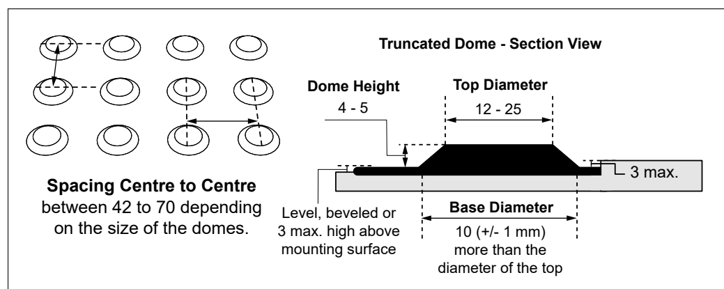
Figure 29: Truncated Domes Specification
