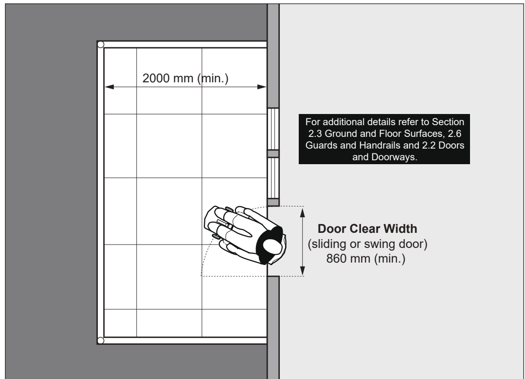
Figure 97: Balcony / Terrace - Plan View
