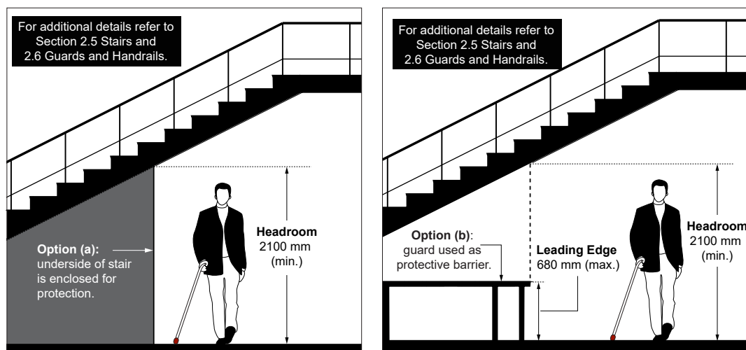
Figure 26: Protection Options Underneath Stairs
