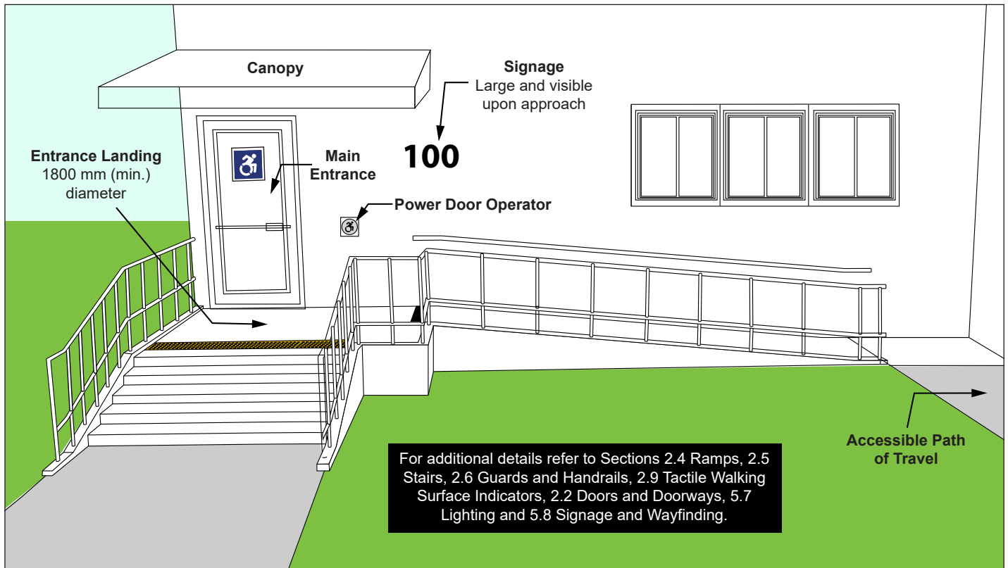
Figure 1: Main or Primary Entrance Features
