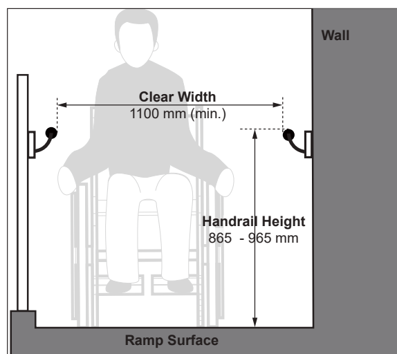
Figure 20: Handrail Design and Features - Section View
