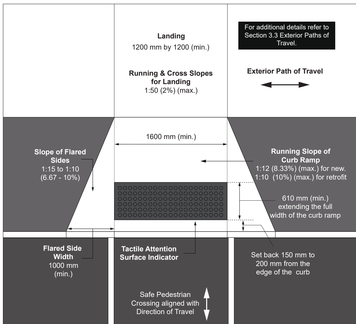
Figure 45: Typical Curb Ramp with Flared Sides Design - Plan View
