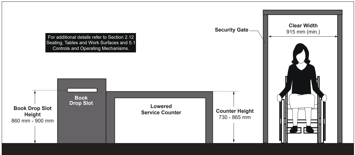
Figure 91: Library Security Gate, Service Counter and Book Drop Slot - Elevation View
