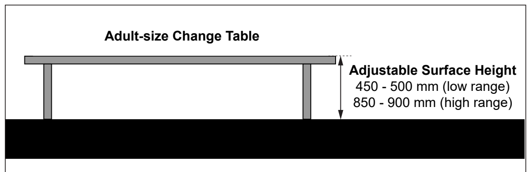
Figure 61b: Adult-Size Change Table
