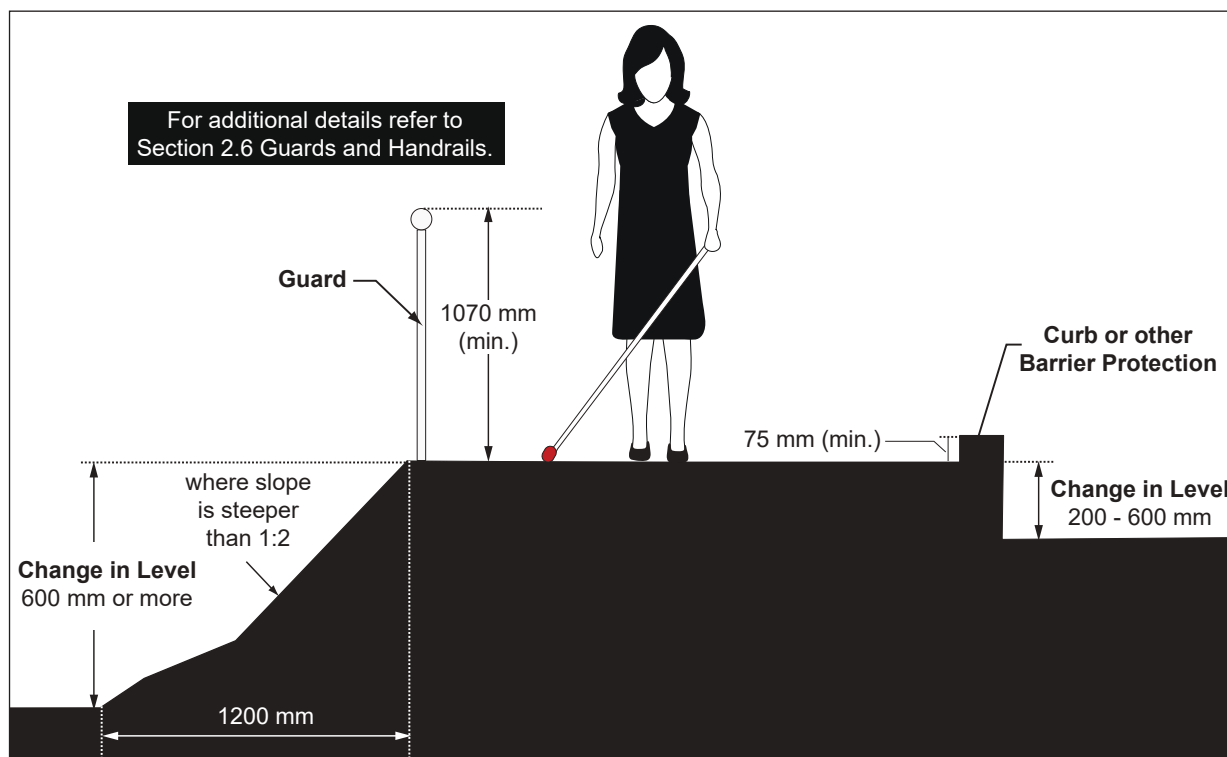
Figure 42: Changes in Level - Edge Protection and Guard Requirements - Section View
