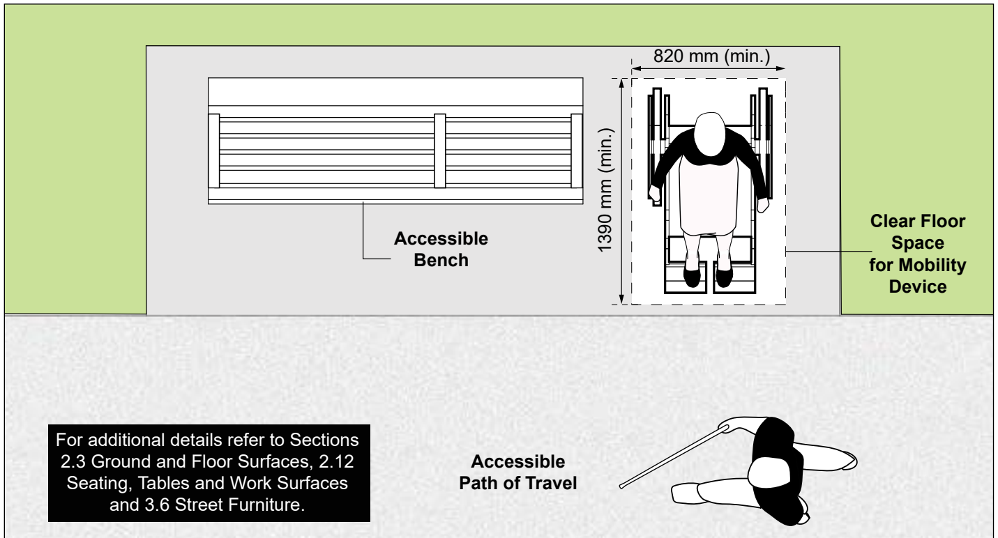
Figure 28: Rest Area - Plan View
