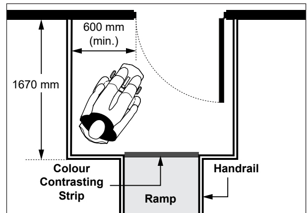
Figure 18a: Door Swings into Ramp Landing
