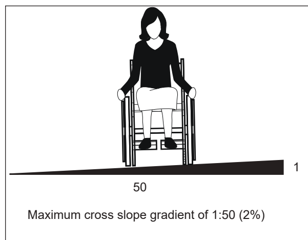
Figure 41b: Cross Slope
