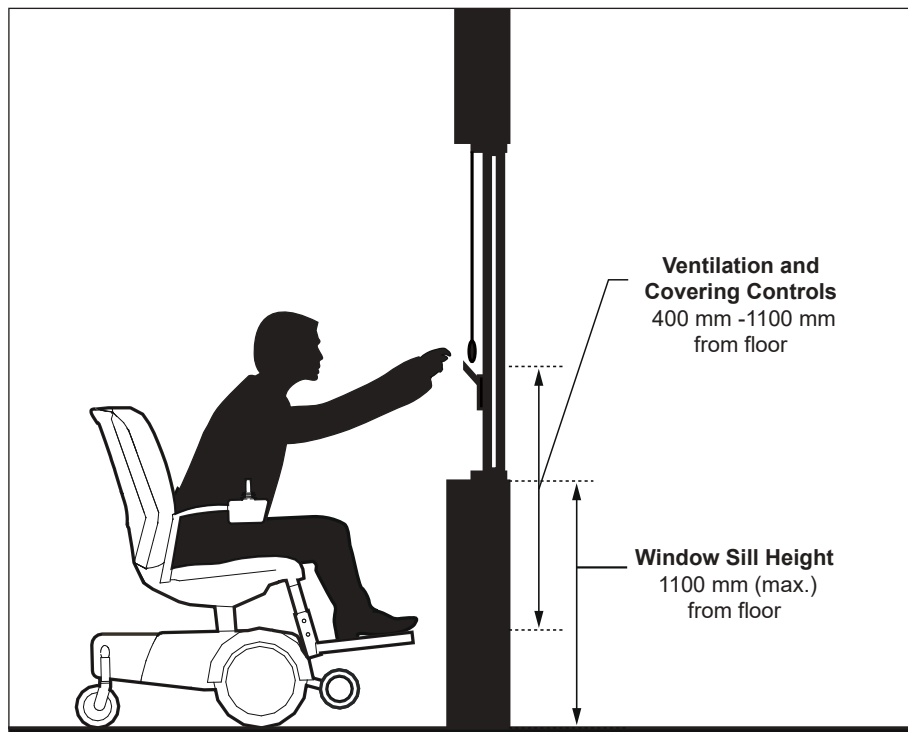
Figure 79: Window Design Features - Elevation View
