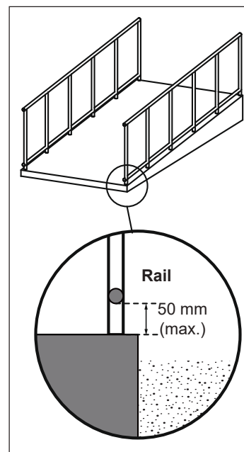
Figure 16c: Rail Protection
