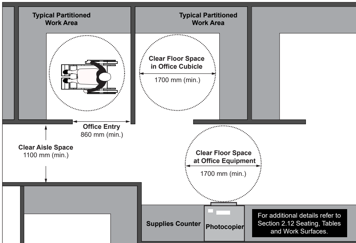
Figure 93: Common-Use Work Areas - Plan View
