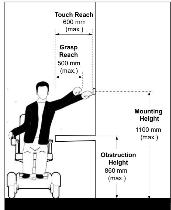
Figure 67b: Maximum Mounting Height over an Obstruction of 860 mm (maximum) for Side Approach and Reach
