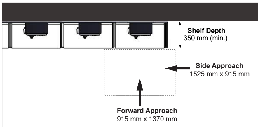
Figure 33: Clear Floor Space Requirements at Accessible Public Telecom Amenity
