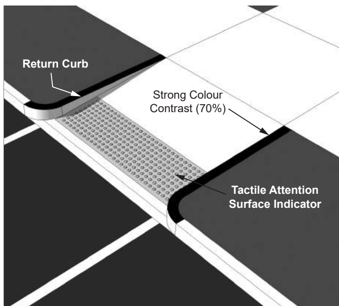
Figure 44b: Curb Ramp with Return Curb
