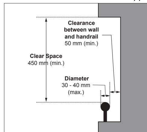
Figure 25b: Handrails in Recessed Area
