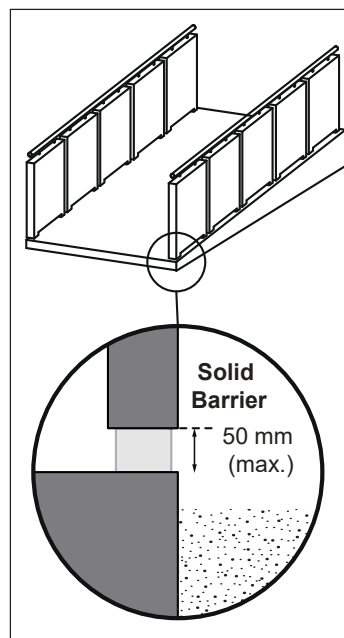
Figure 16b: Solid Barrier Protection
