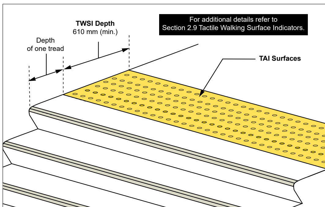
Figure 23: TAI Surfaces at Top of Stairs
