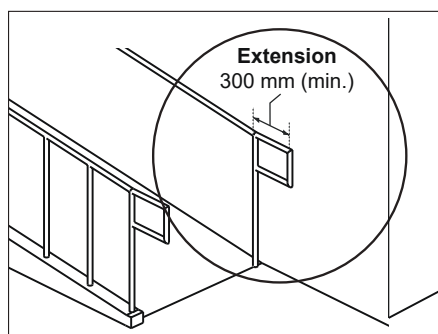
Figure 19a: Handrail Returns to Guard or Rail
