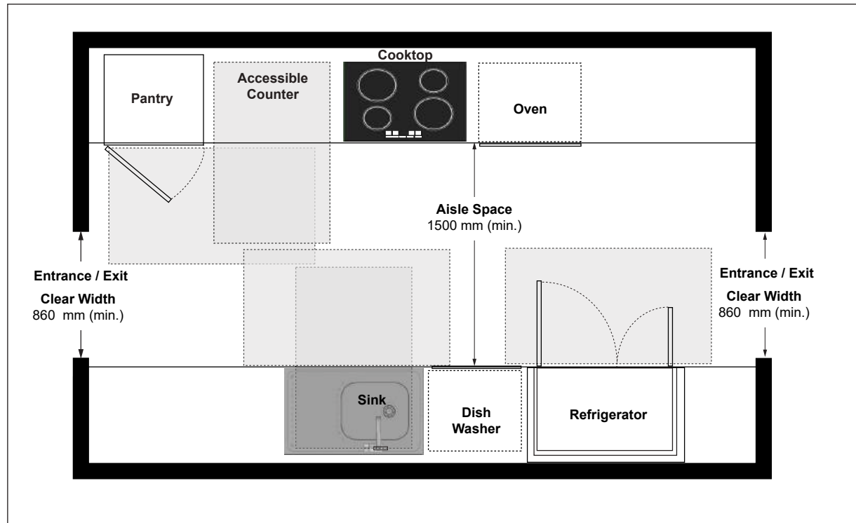
Figure 85: Pass-Through or Galley Kitchen - Plan View
