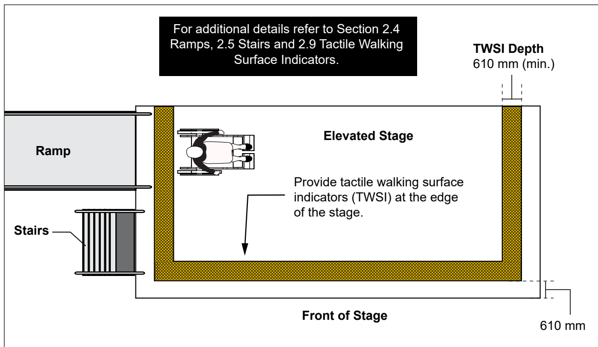
Figure 101: Elevated Platform or Stage - Plan View
