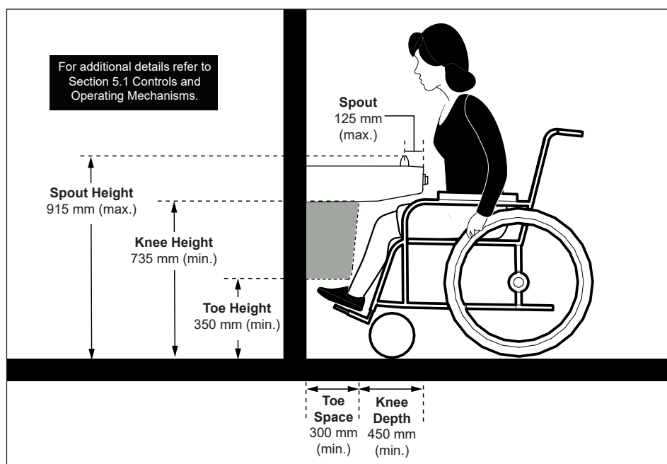
Figure 32: Drinking Fountain Design and Layout - Elevation View
