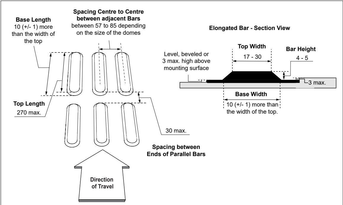
Figure 30: Elongated Bars Specification
