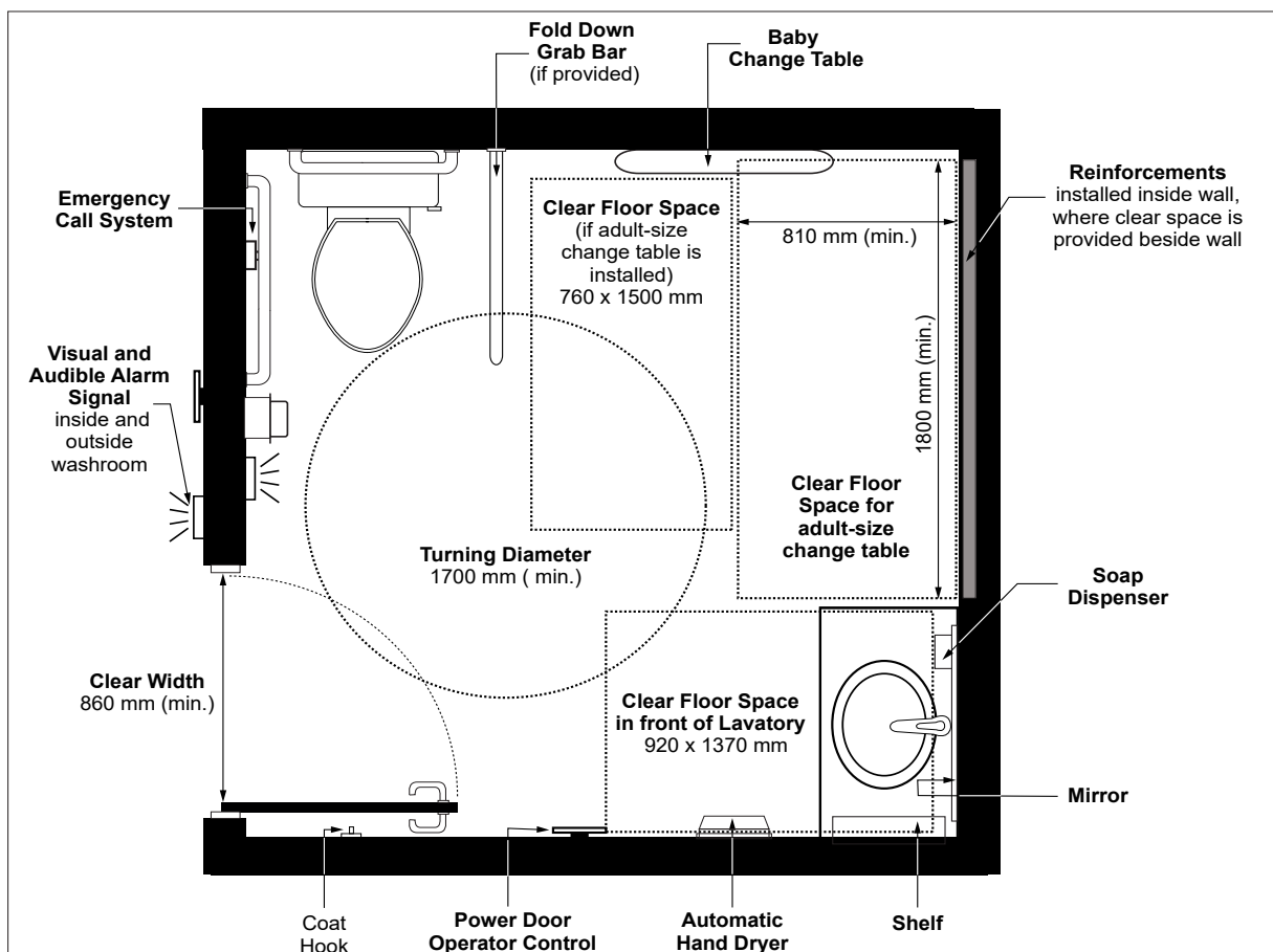
Figure 53: Universal Washroom
