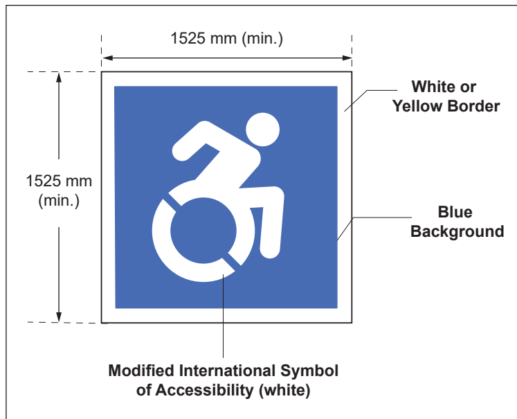
Figure 39: Accessible Parking Pavement Marking
