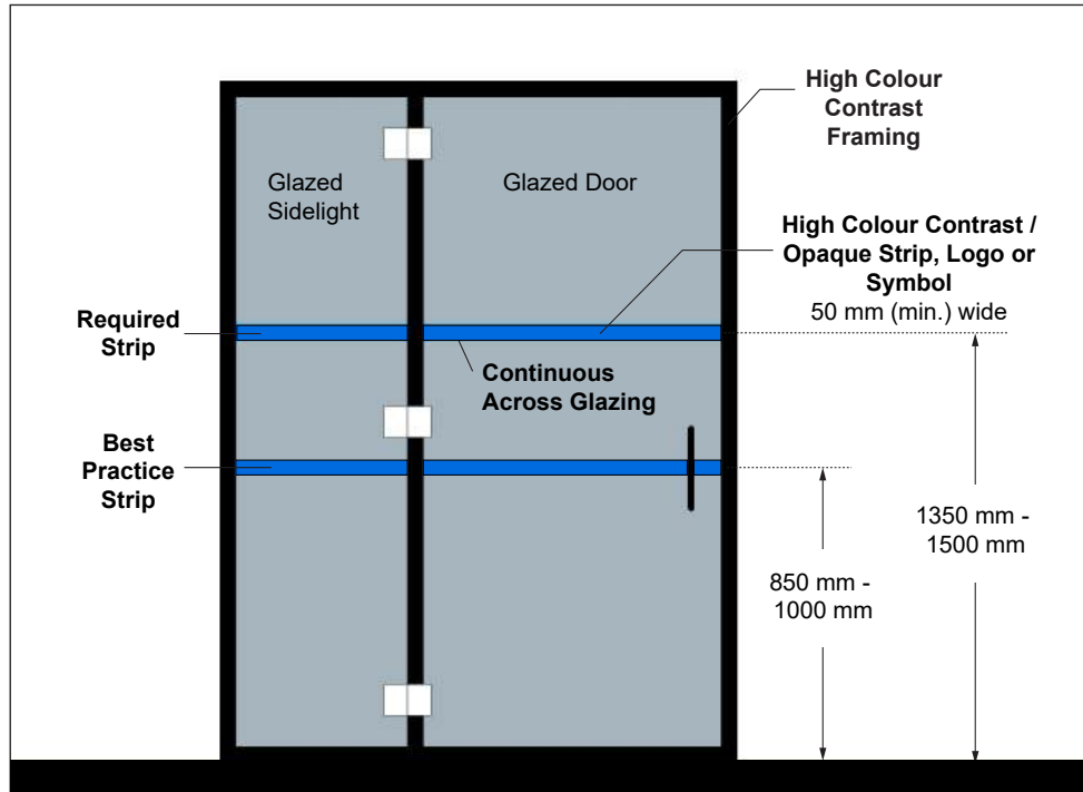
Figure 11: Glazed Doors - Elevation View
