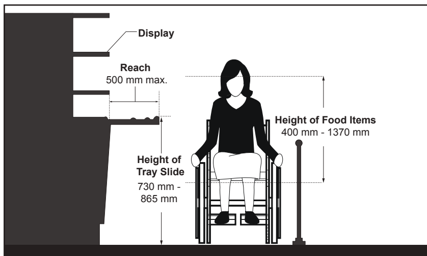
Figure 84a: Food Displays and Tray Slides - Section View
