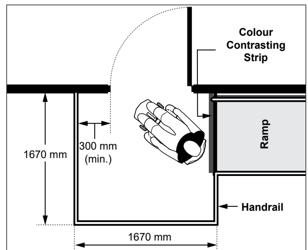
Figure 18b: Door Swings Away From Ramp
