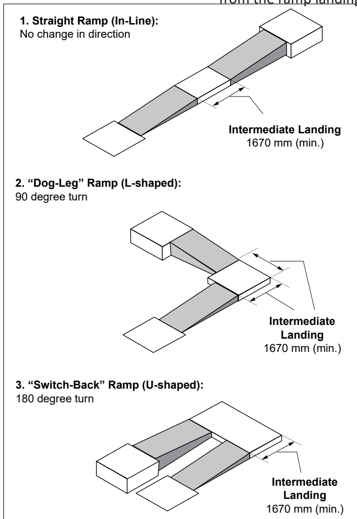
Figure 17: Typical Ramp Configurations
