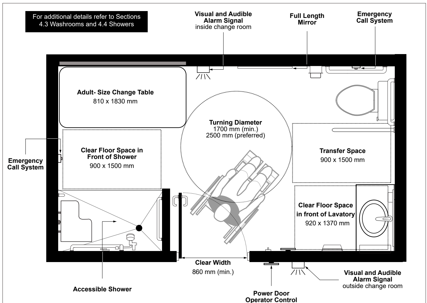
Figure 95: Universal Change Room
