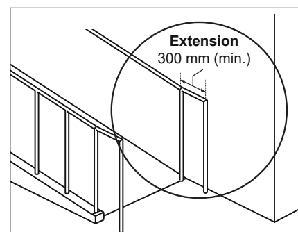
Figure 19c: Handrail Returns to Floor
