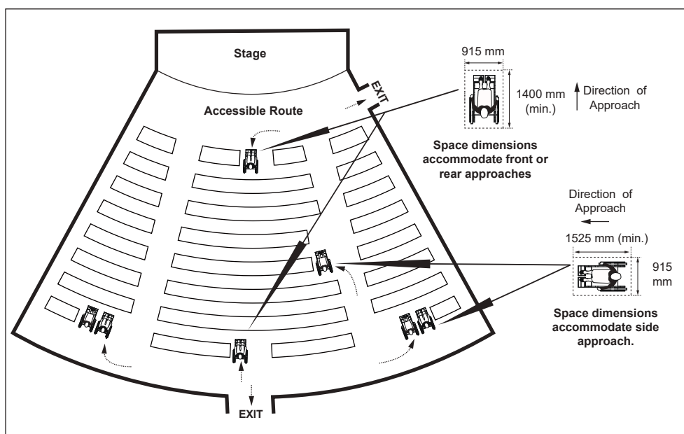
Figure 82: Accessible Seating Plan - Example of Viewing Positions
