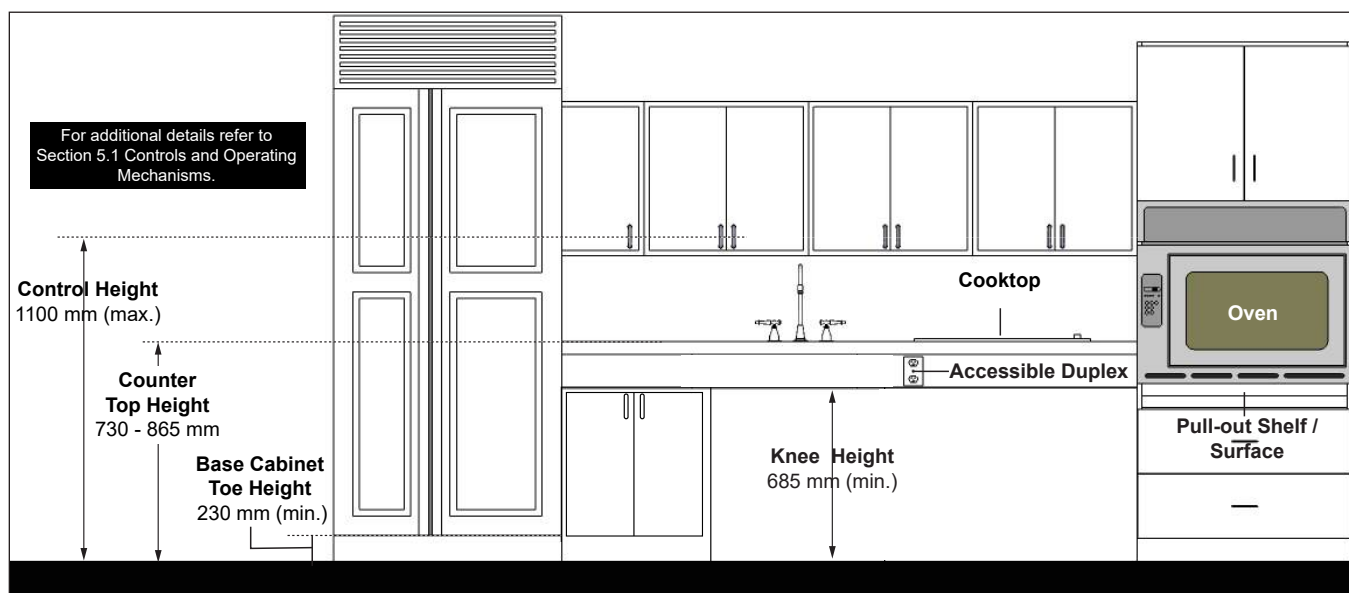
Figure 88: Kitchen Amenities
