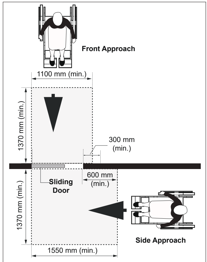
Figure 9b: Front and Side Approach at Sliding Door - Plan View
