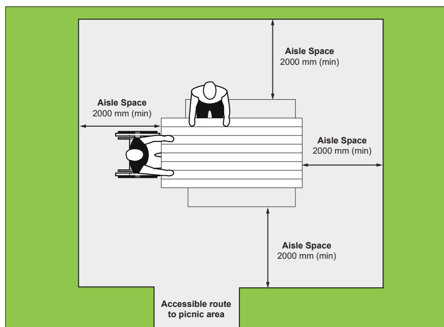
Figure 102a: Picnic Table Design and Features - Plan View
