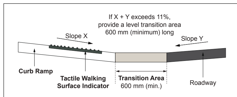
Figure 43: Transition Area - Counter Slope
