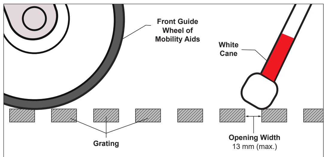
Figure 14b: Gratings - Section View
