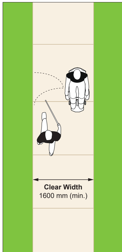
Figure 40a: Minimum Clear Width of Exterior Path of Travel
