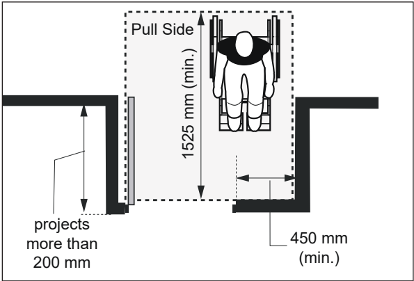
Figure 8a: Pull Side Approach at Recessed Side-Hinged Door - Plan View
