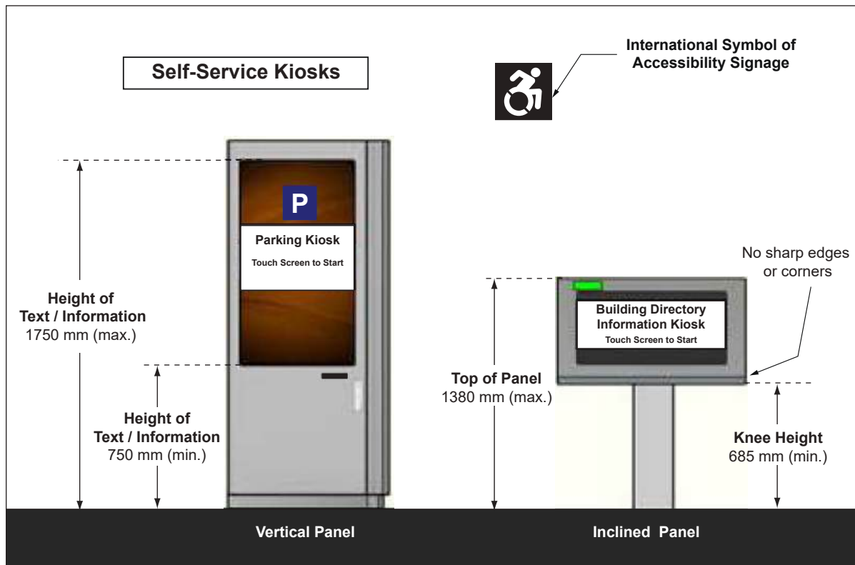
Figure 78: Self-Service Kiosks - Elevation View
