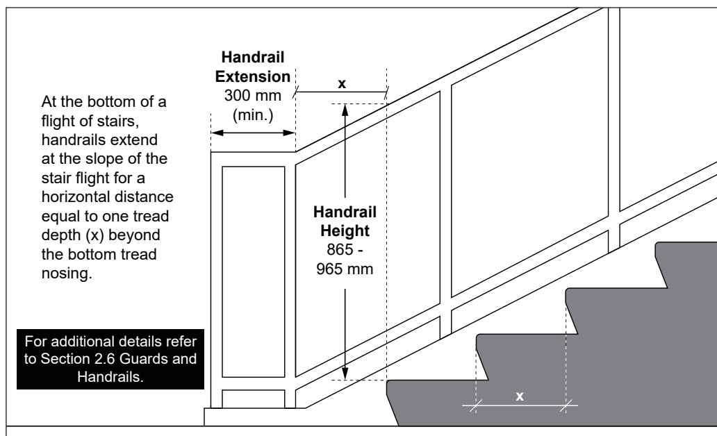
Figure 24: Handrail Extensions at Stairs - Section View
